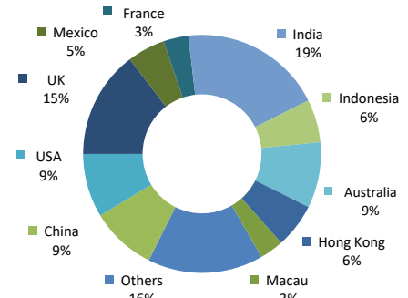
GEOGRAPHICAL EXPOSURE 5
