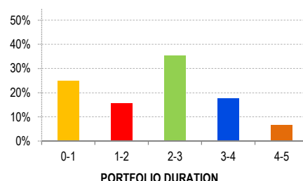
PORTFOLIO DURATION
