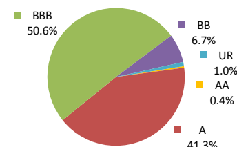
RATING PROFILE
